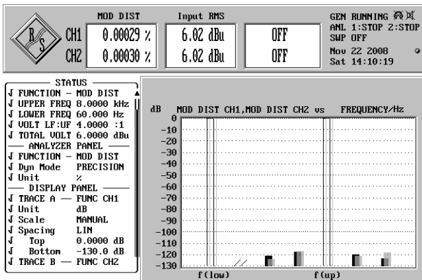
Intermodulation distortion 8kHz/60Hz Ratio: 4:1 SSOM-04Mb
