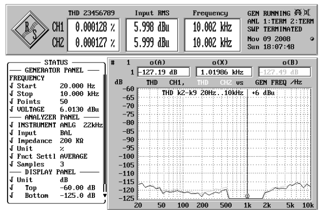
THD k2.k9 von 20 Hz...10 kHz (400 Hz-Tip comes from Analyzer)
