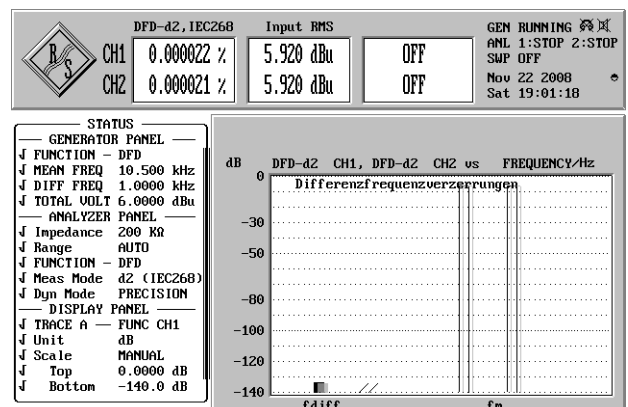
Differential frequency distortion 10,5 kHz Diff.=1 kHz SSIM-04Mb
