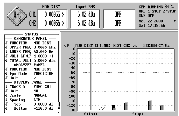
Intermodulation distortion 8 kHz/60 Hz Ratio: 4:1 SSIM-04Mb
