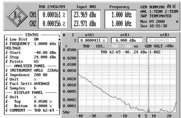
THD k2.k9 above levels of -40 dBu...+24 dBu SSIM-04Mb
