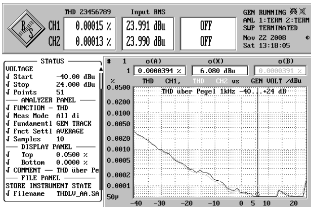
THD k2.k9 above levels of -40 dBu...+24 dBu SSOM-04Mb
