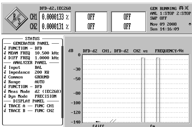
Differential frequency distortion 10,5 kHz, Diff.=1 kHz SSOM-04Mb
